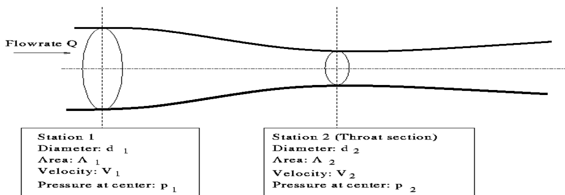
Figure 4: Principle Venturi effect
